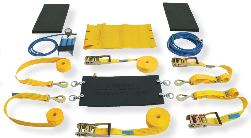
Set LDS 45 x 23 with swivel eyelets
