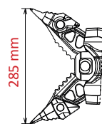
Spreader tip Part-no. 1050616
